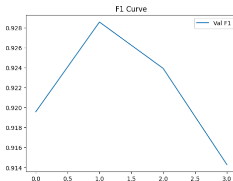
(A) IndoBERT
