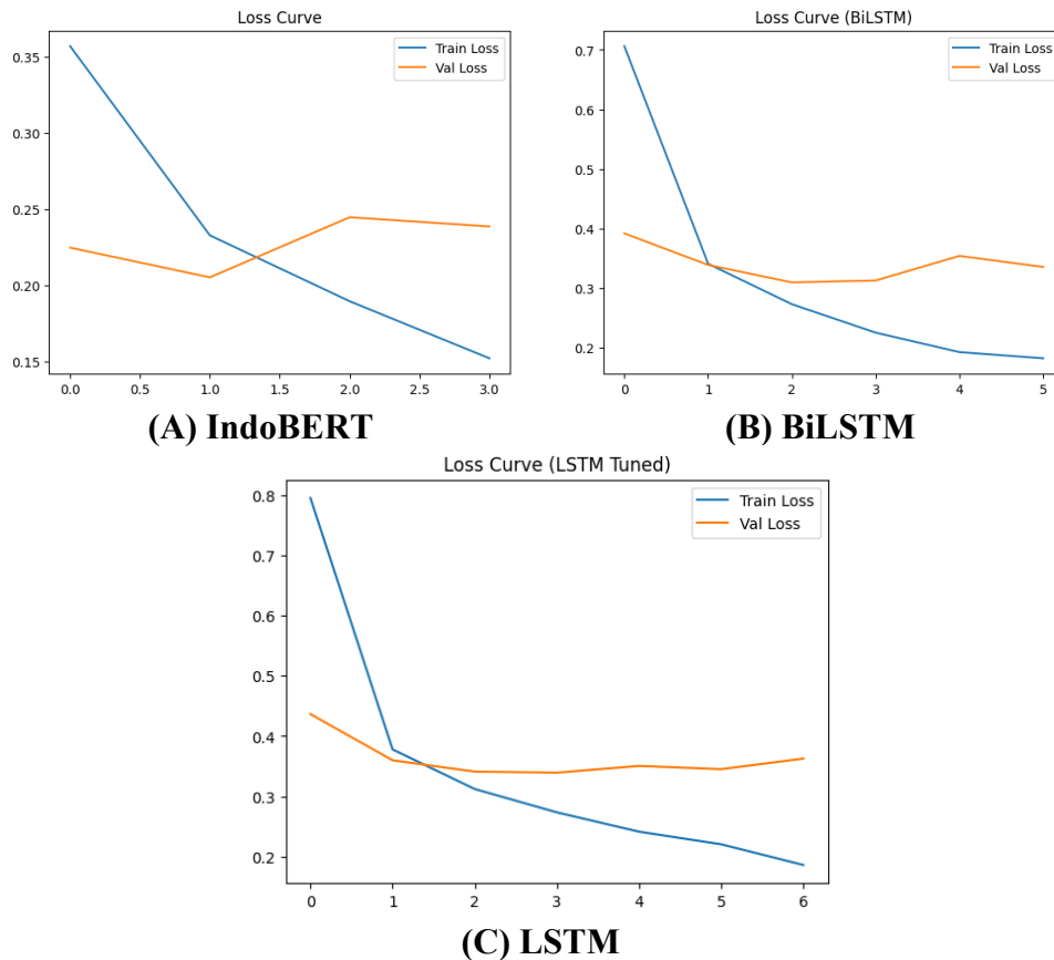
Gambar 1. Loss Curve
