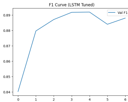
(C) LSTM
